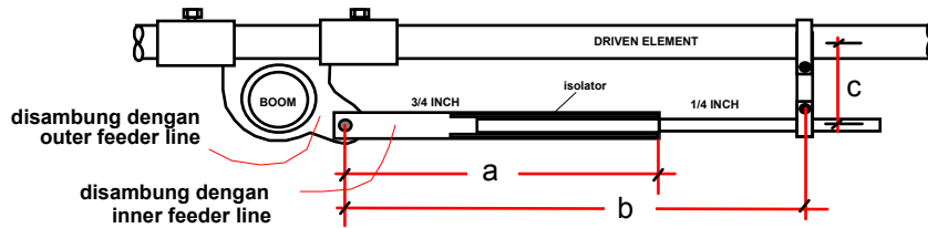
GAMMA MATCHING DEVICE Gambar 7
