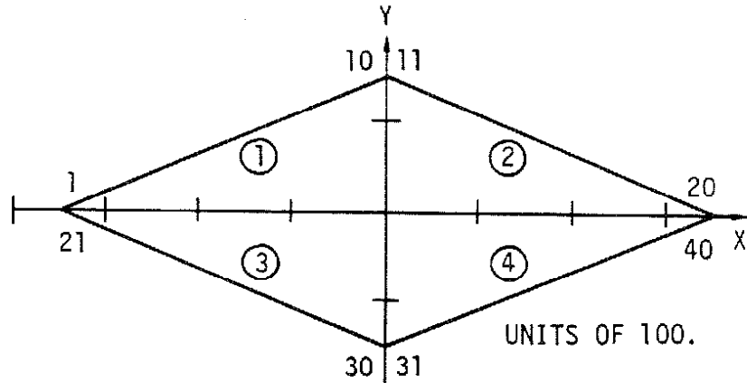
Figure 7. Rhombic Antenna - No Symmetry.
